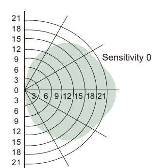
Wall Pattern (Unit: m) Installation Height: 5m
