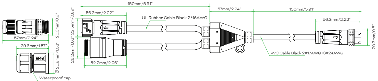
RJ45 Power Injector Cable Kit (Connector included)
