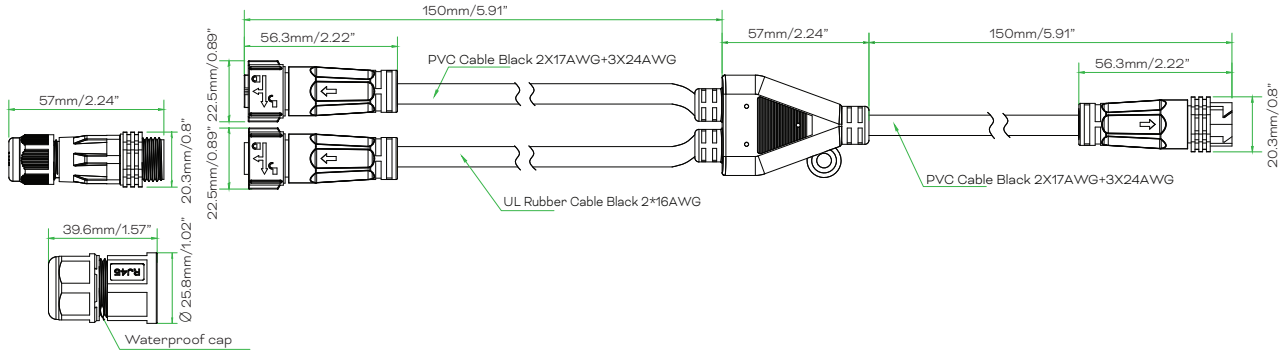
RJ45 Power Injector Cable Kit (Connector included)
